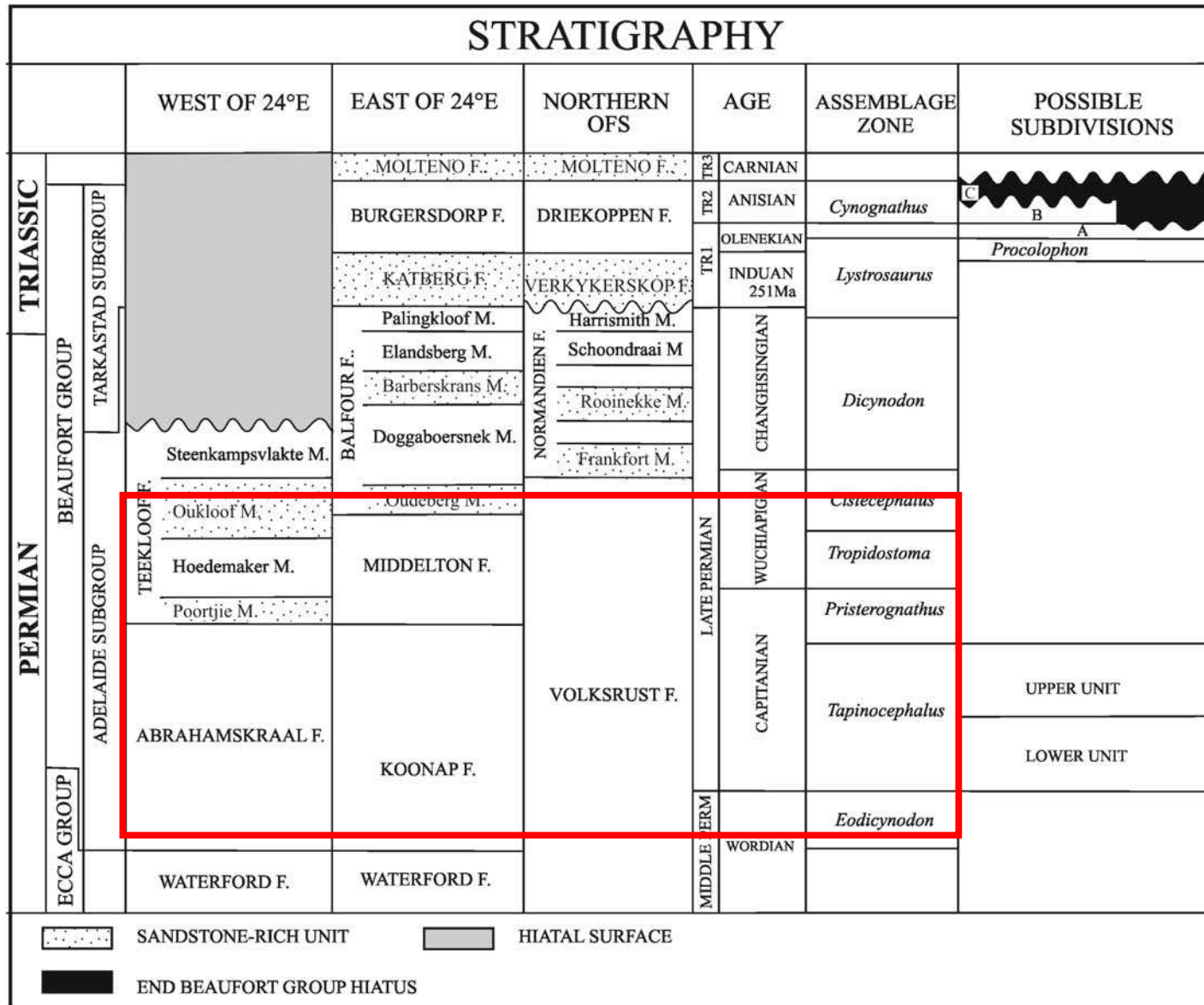
Fig. 7. Beaufort Group stratigraphy showing relationship between fossil assemblage zones and formations represented in the TCP study area (red rectangle) (Catuneanu et al. 2005). Note that the dating of these units as shown here has since been modified. For example, the Mid / Late Permian boundary is now placed at the top of the Pristerognathus Assemblage Zone.
