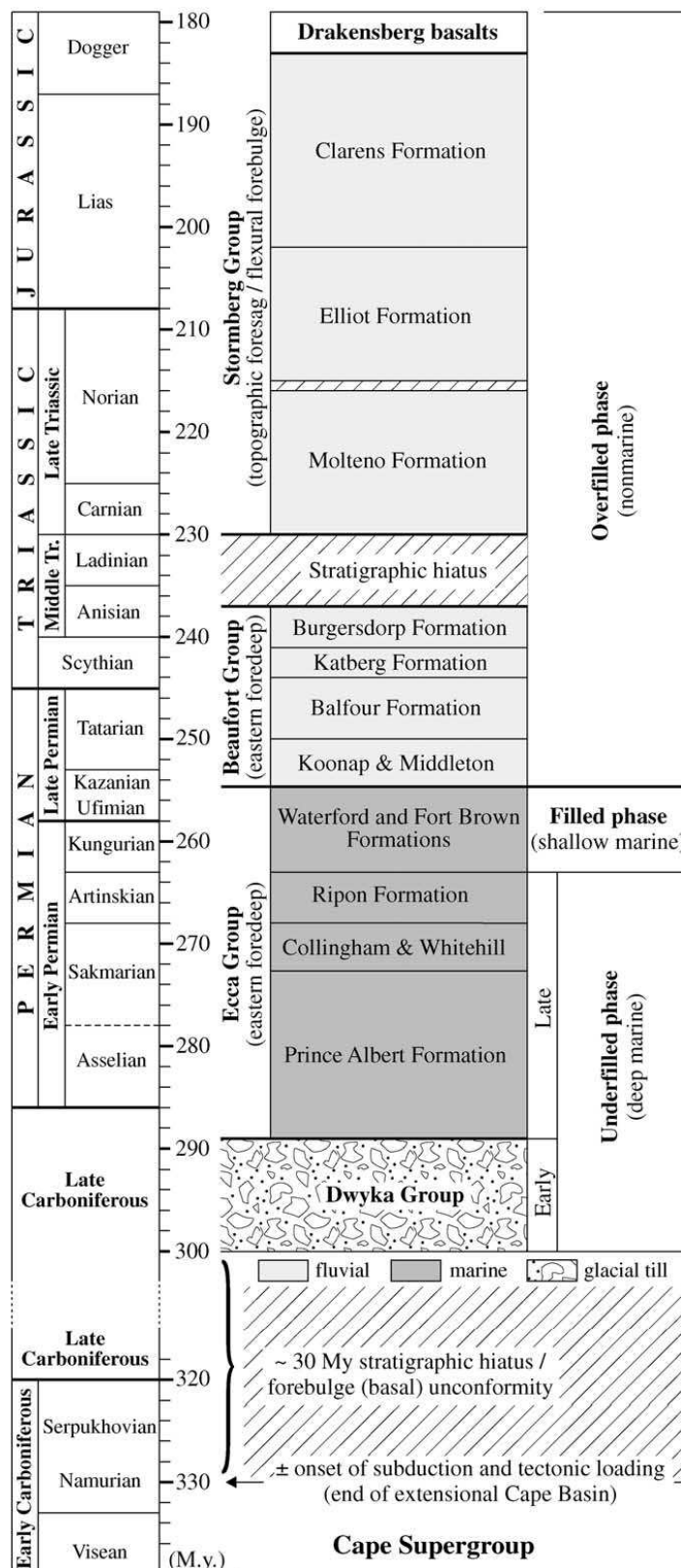
Fig. 4. Stratigraphic subdivision of the c. 12km-thick Karoo Supergroup (From Catuneanu et al. 2005). The bold red line emphasizes the Late Carboniferous to Late Permian sedimentary units represented in the TCP study area. Not all relevant formations are shown here (See Fig. 5).
